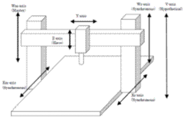
Fig. 5.1 (a) Example of machine structure
